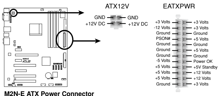
M2N-E ATX Power Connector
