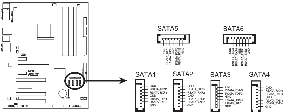
M2N-E SATA-Anschlüsse
