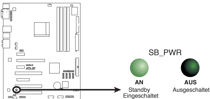
M2N-E Onboard-LED
