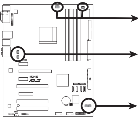
M2N-E Lüfteranschlüsse
